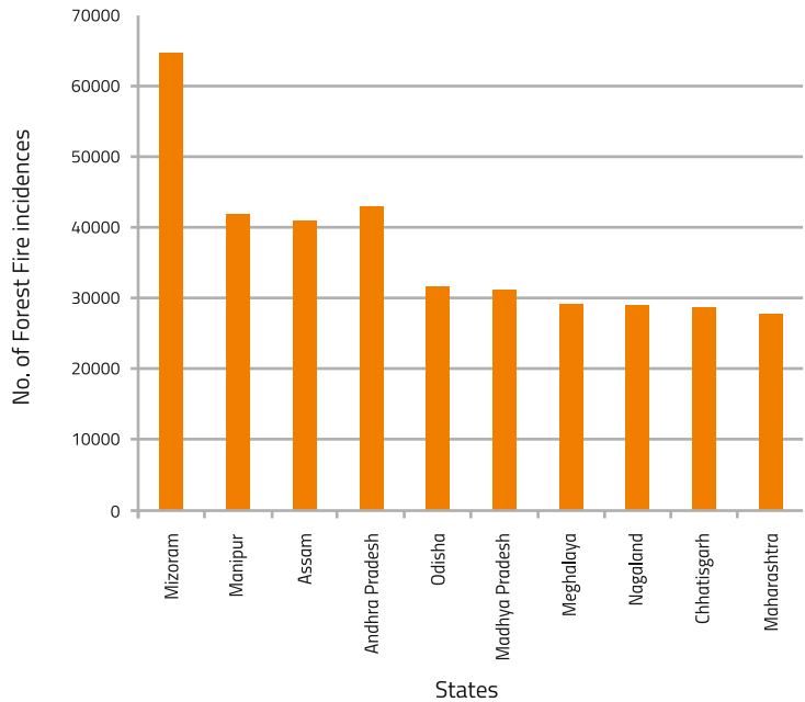
Number of Forest Fire Incidences in Top Ten Fire Impacted States of India (2001-2016)
